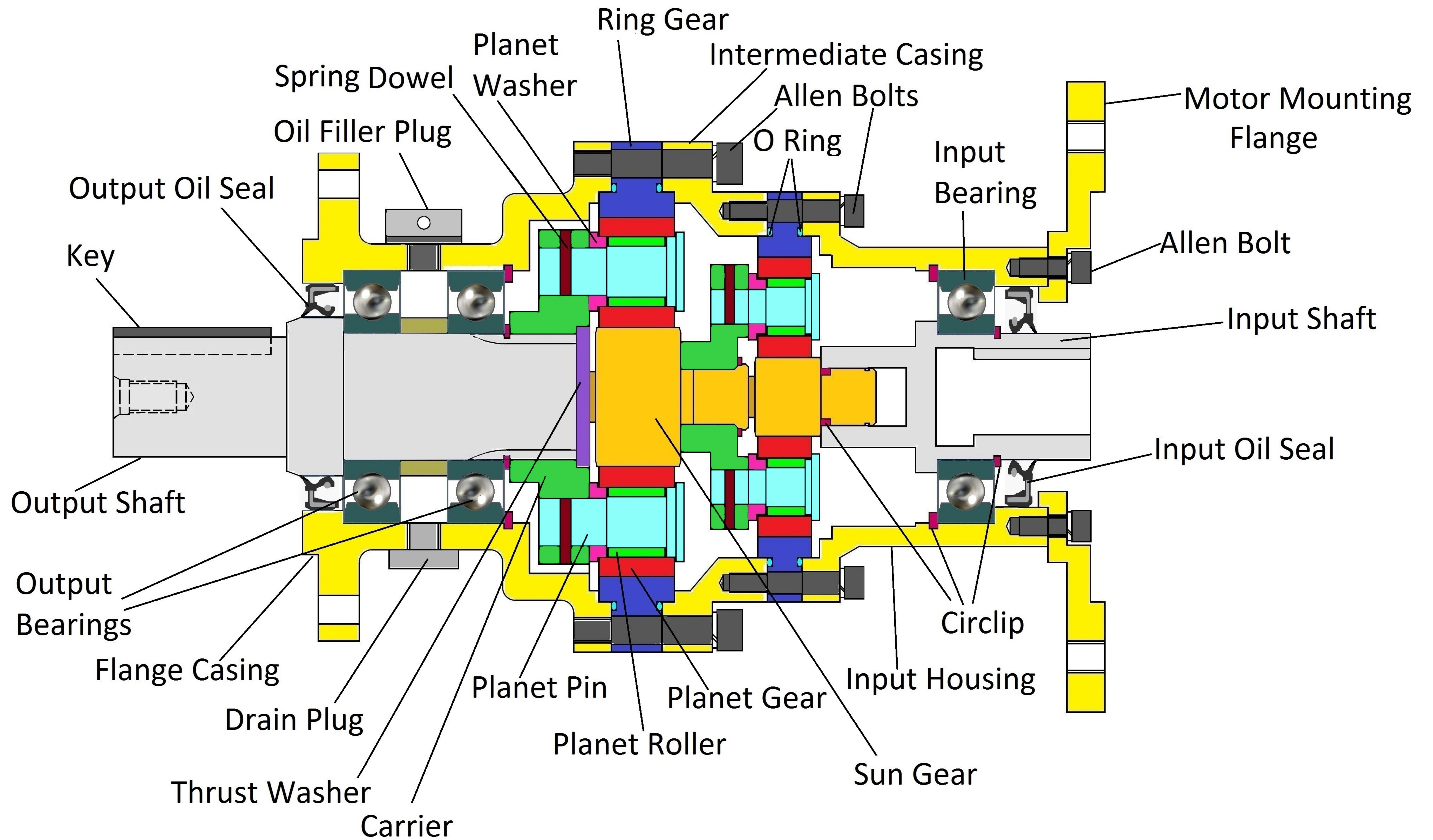
Planetary Gearbox
