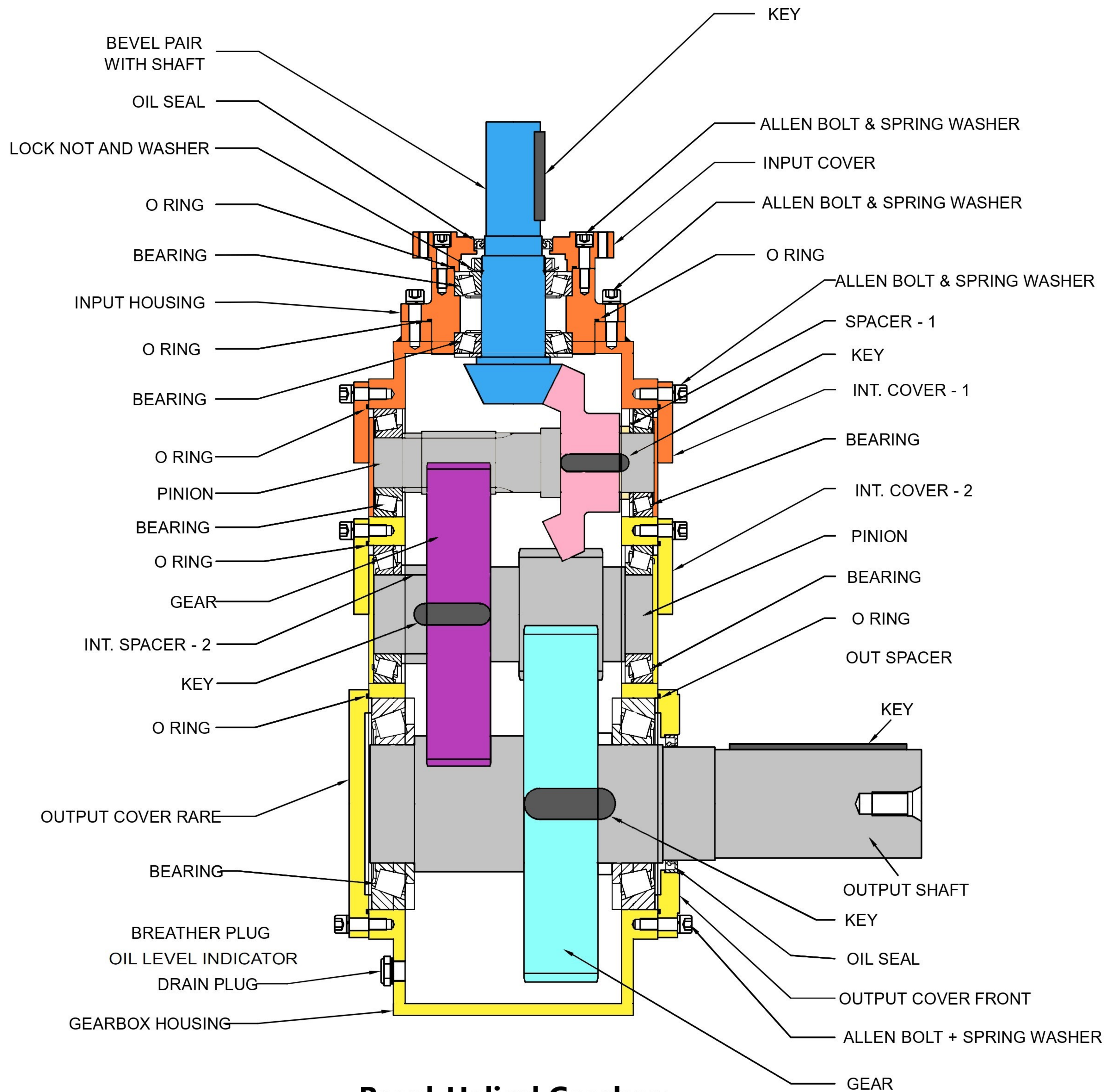
Bevel-Helical Gearbox
