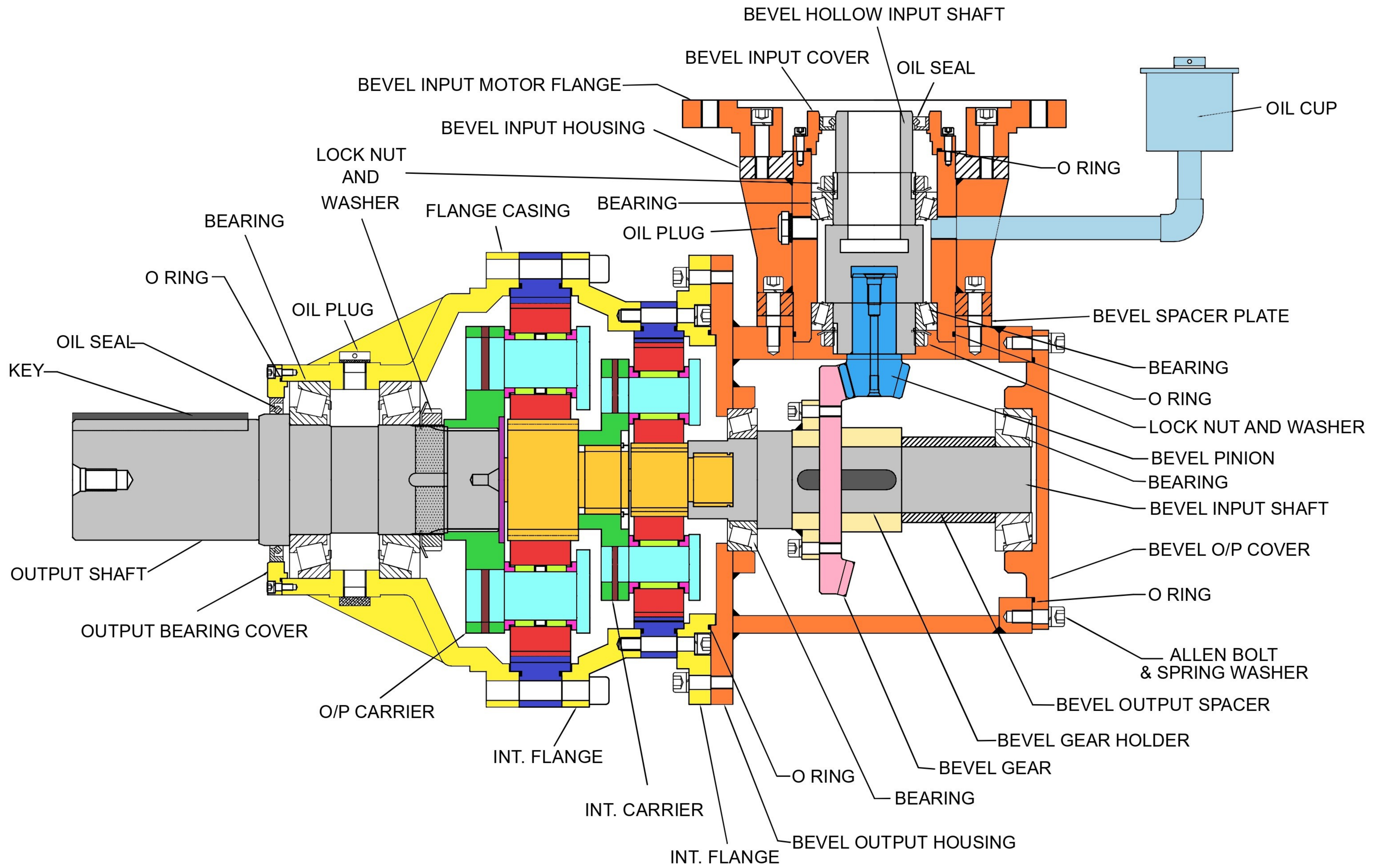
Bevel-Planetary Gearbox
