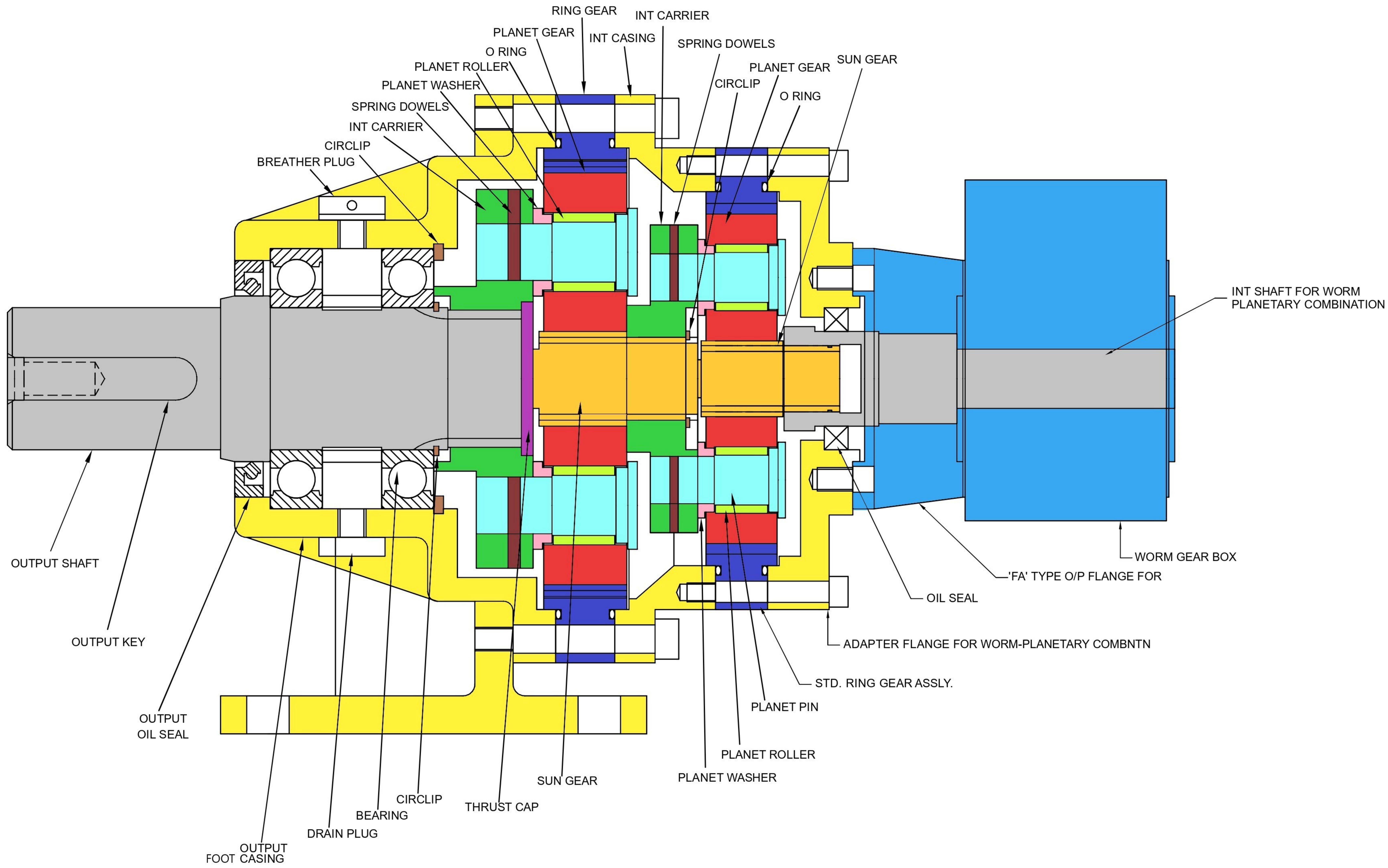
Worm-Planetary Gearbox
