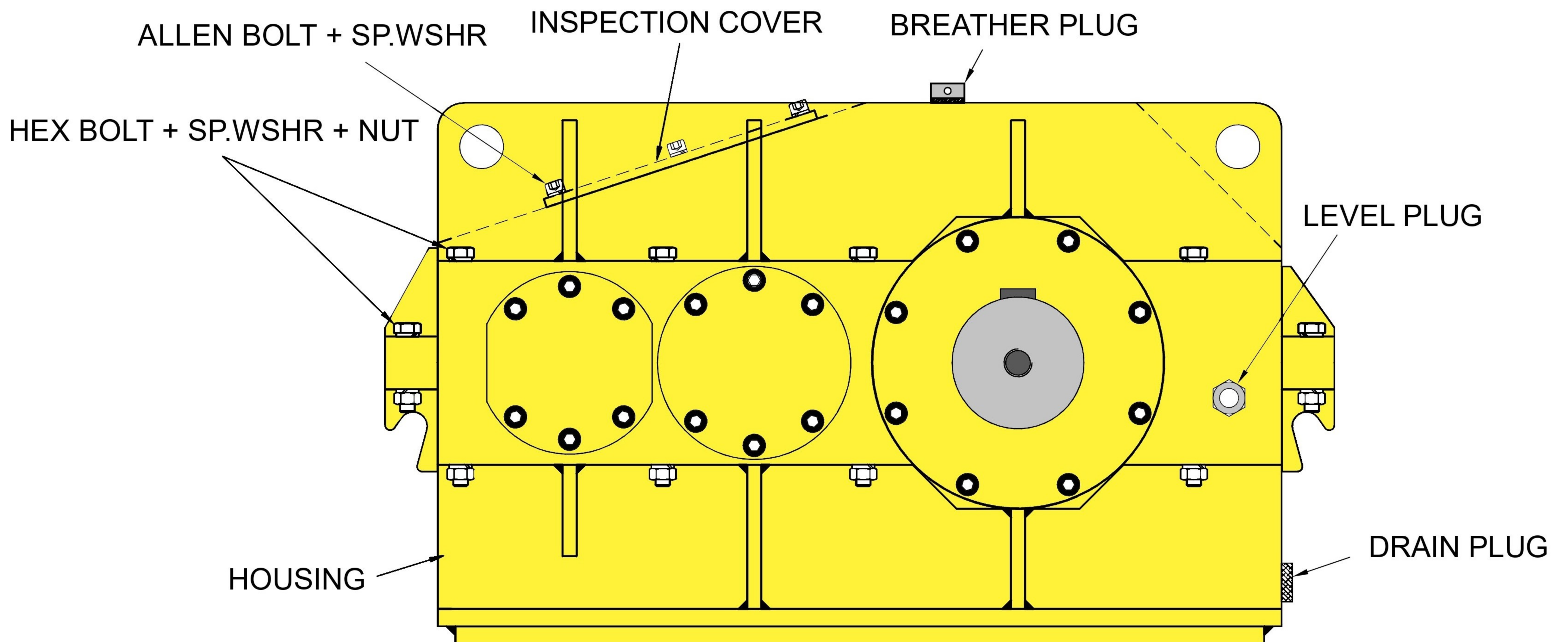
FRONT VIEW (OUTPUT SIDE)
