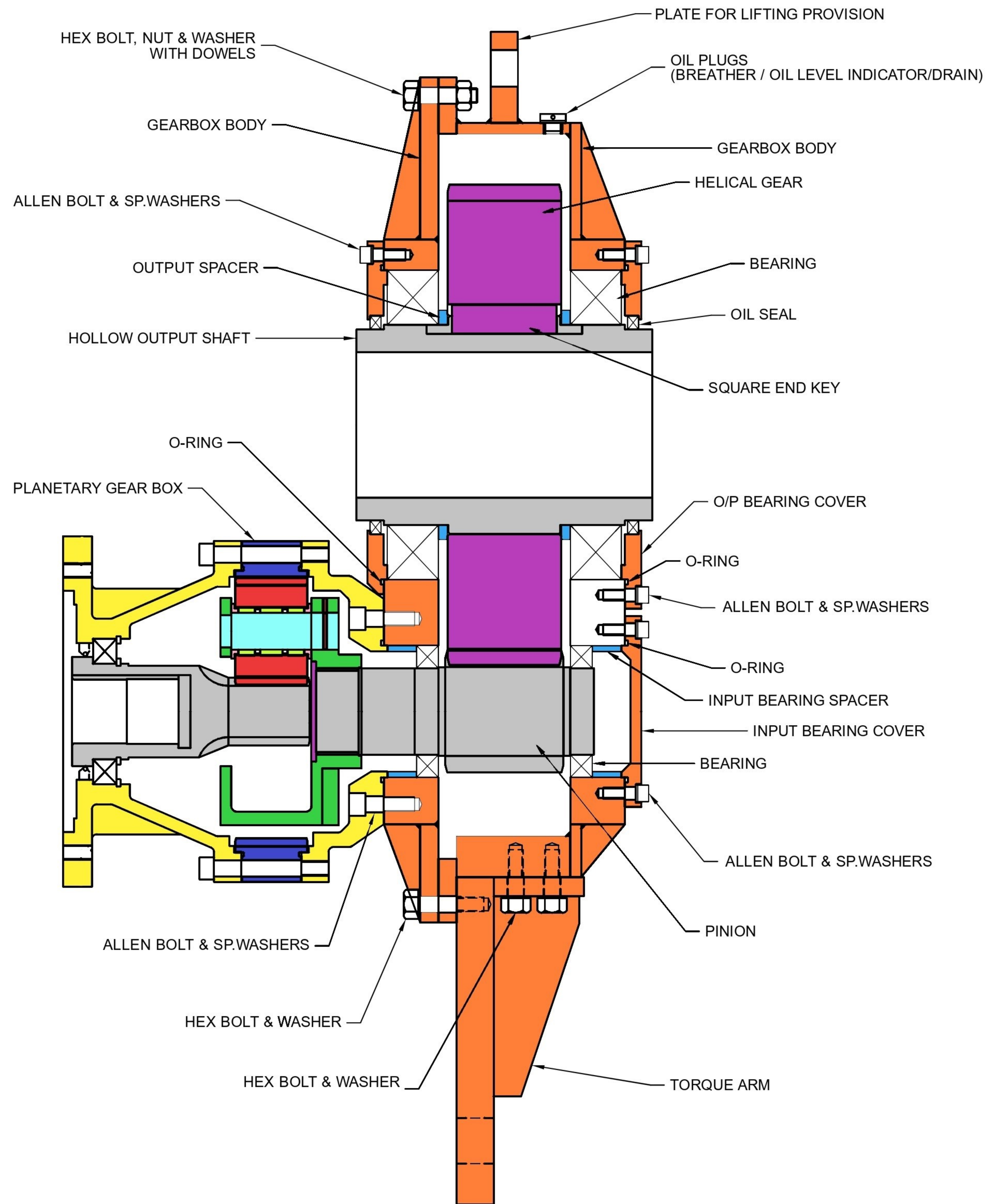
Helical-Planetary Gearbox
