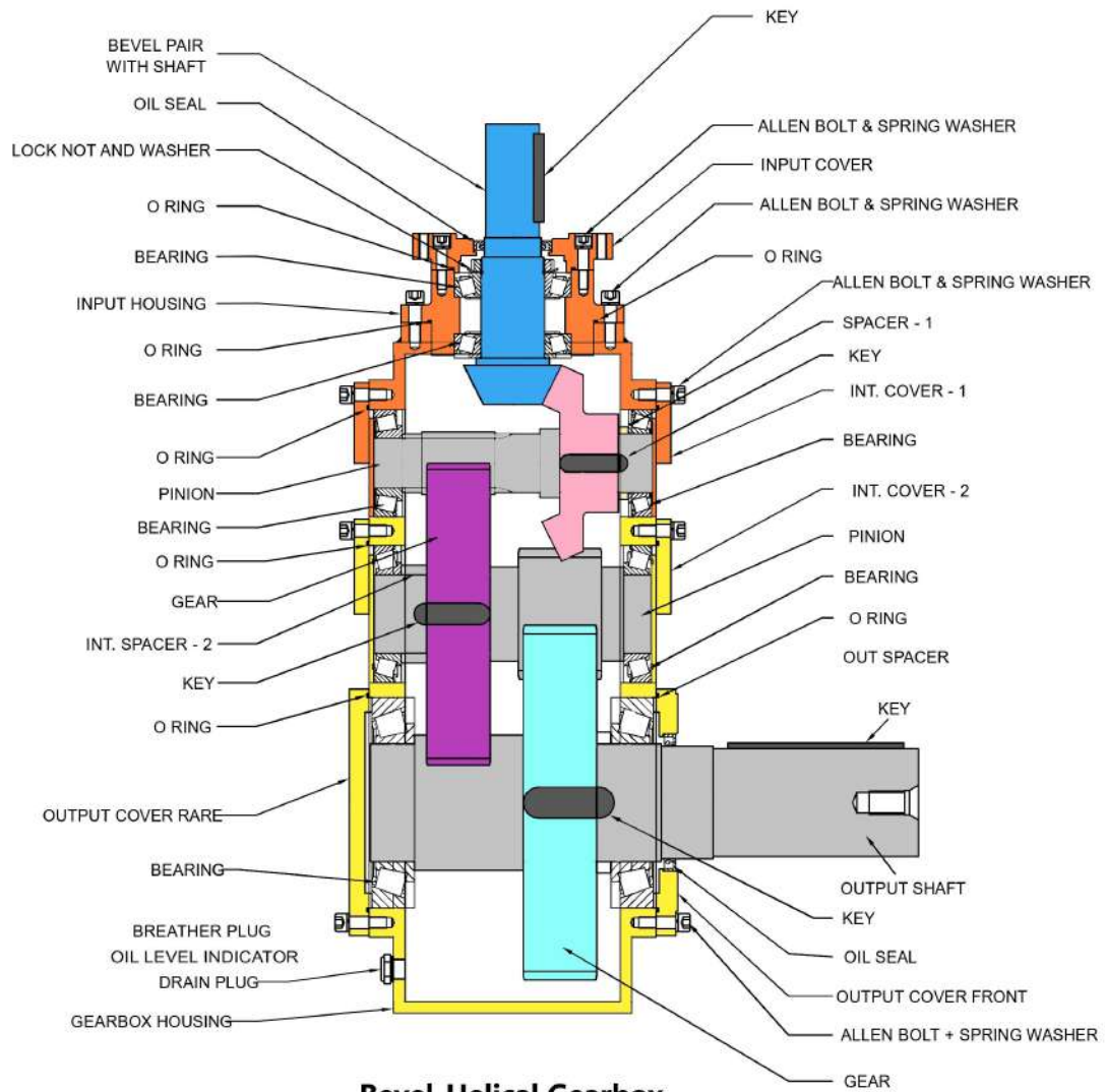
Bevel-Helical Gearbox
