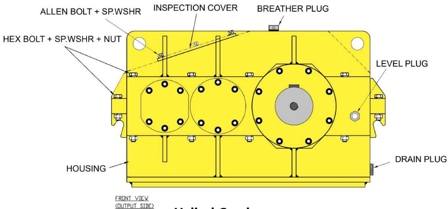
Helical Gearbox
