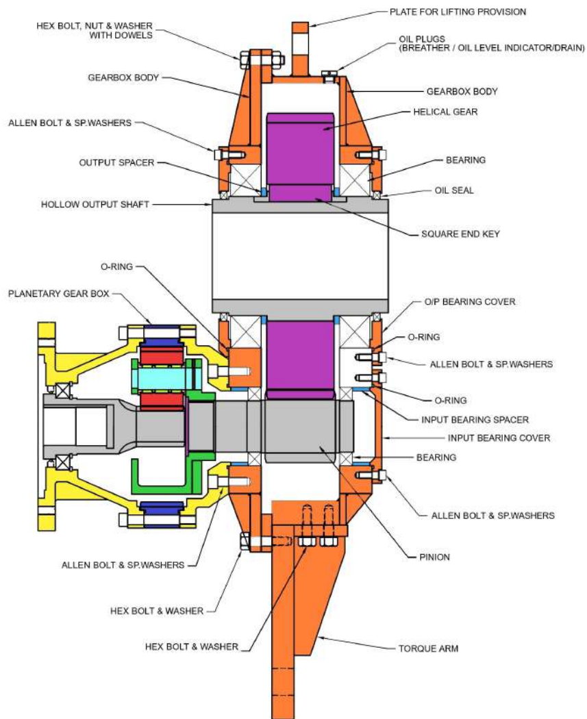
Helical-Planetary Gearbox
