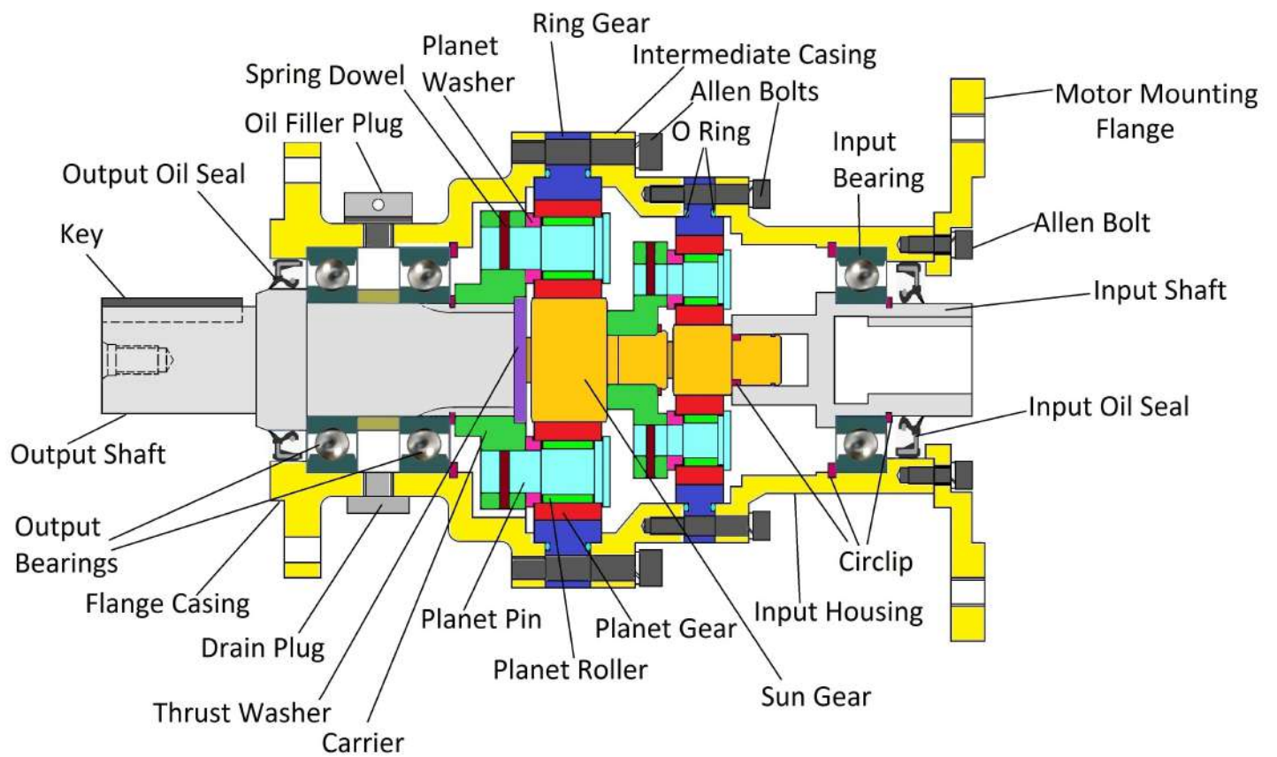
Planetary Gearbox
