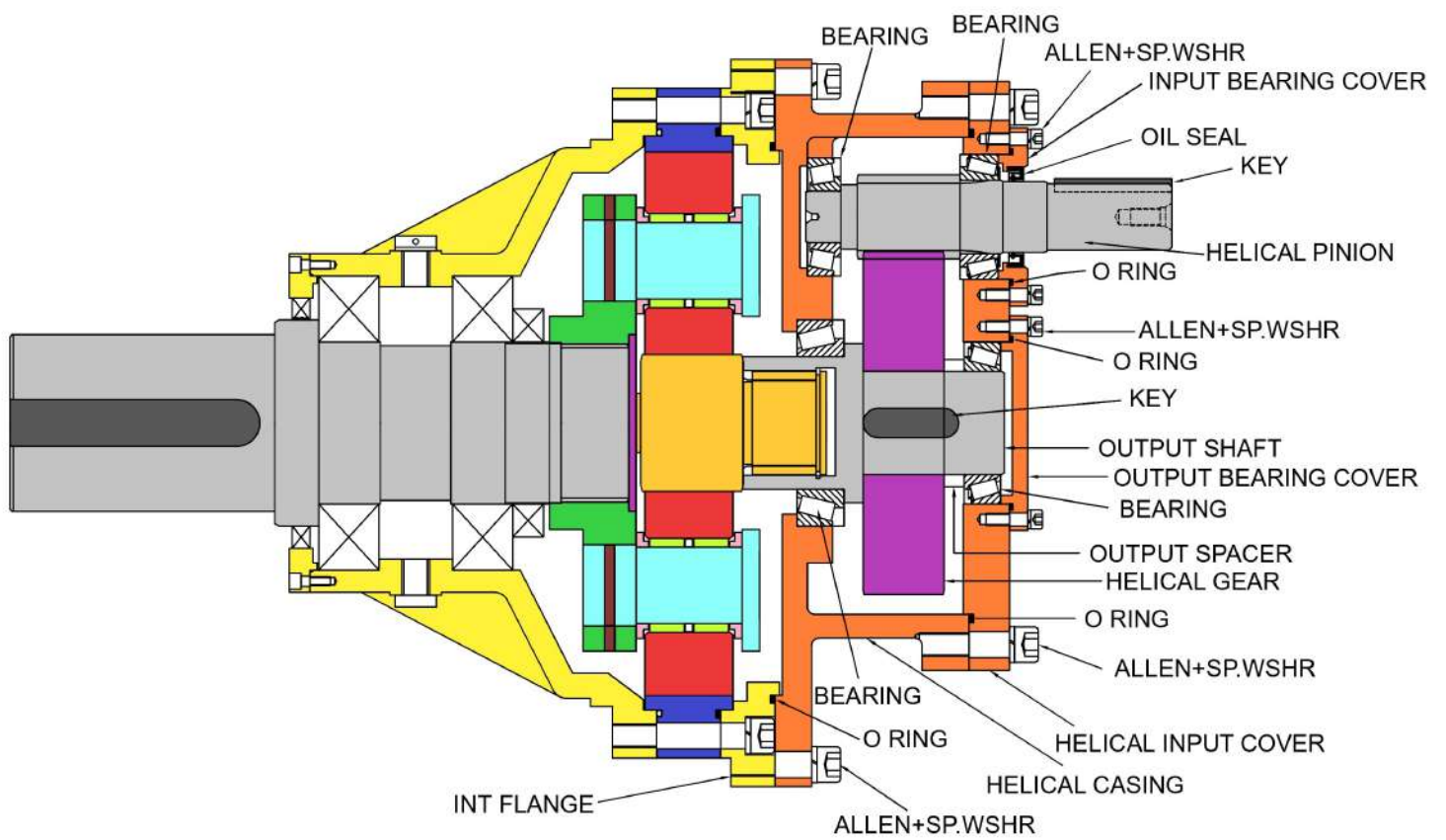
Planetary-Helical Gearbox
